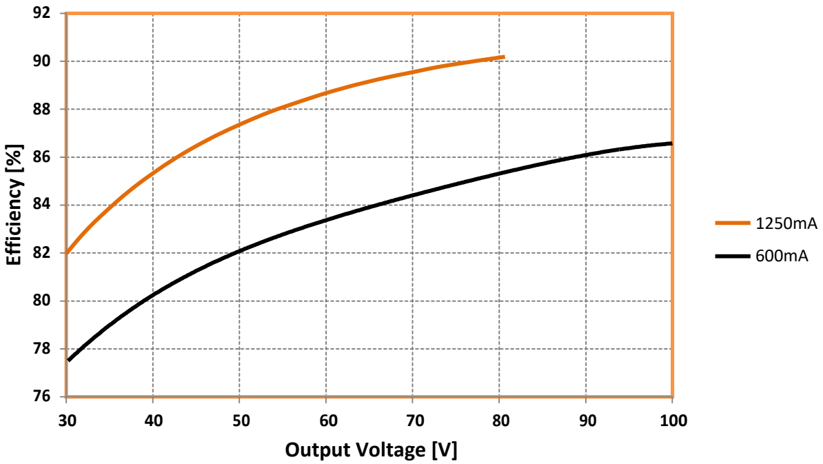
Efficiency @ 277V
