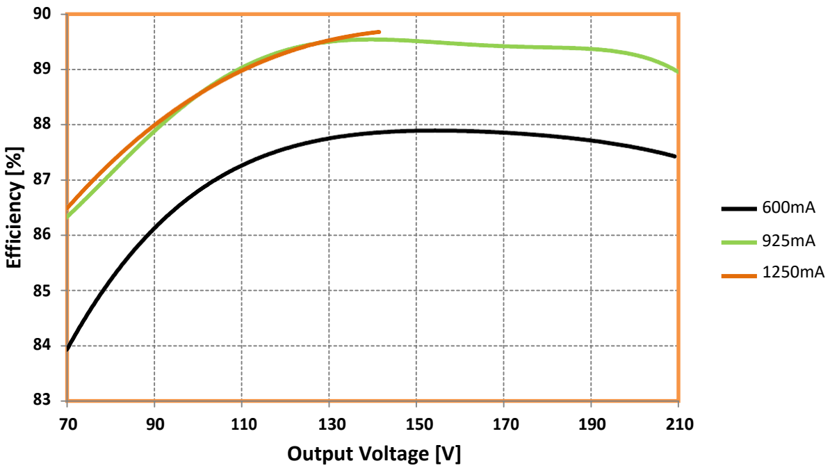
Efficiency @ 120V
